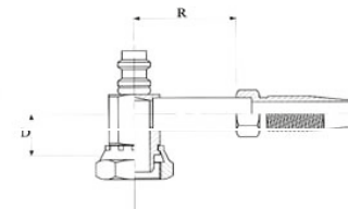
Tube "O" compressor wartel, 90° / R134 ventiel Tube "O" compressor fitting, 90° / R134 valve Raccord tube "O" compresseur, 90° / R134 valve
