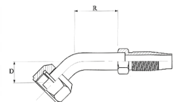
Long pilot "O" ring wartel, 45° - pijp aansluiting "O" ring female swivel, 45° - tube connection "O" ring femelle tournant, 45° - tube connection
