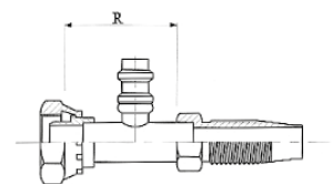
Tube "O" compressor wartel / R134 ventiel Tube "O" compressor fitting / R134 valve Raccord tube "O" compresseur / R134 valve
